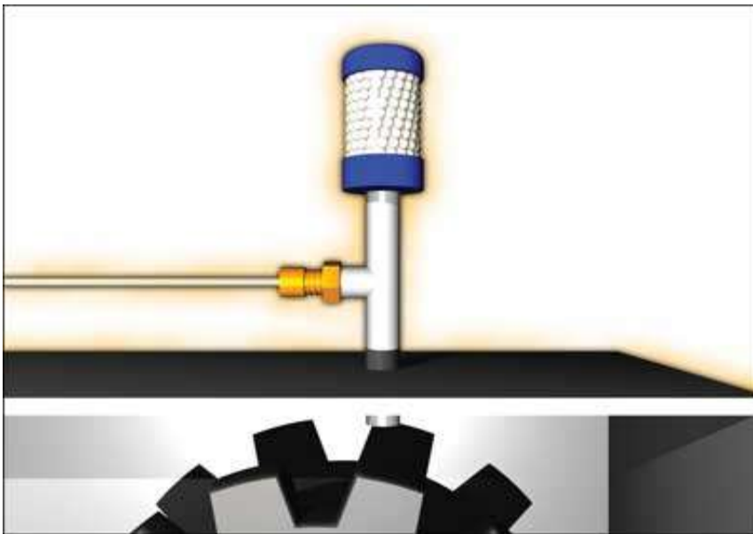
Figure 3 - Spin-On Filter/Breather
